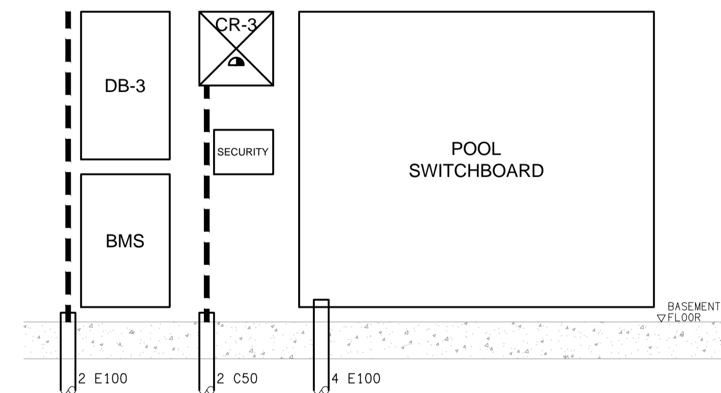
DETAIL B ELECTRICAL EQUIPMENT ELEVATION NOT TO SCALE
